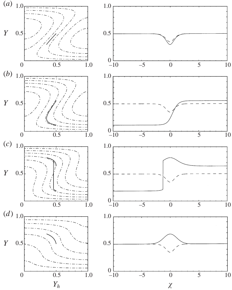
FIGURE 2. Examples of the four types of hydraulic solutions of (3.5) considered by HJH for Y_0 = 0.5 : (a) subcritical ( \epsilon = 0.15 , \alpha = 0.05 , so Fr = 0.2 ), (b) constriction-controlled ( \epsilon = 0.15 , \alpha = 0.1 , so Fr = 0.4 ), (c) approach-controlled ( \epsilon = \alpha = 0.15 , so Fr = 0.6 ) and (d) supercritical ( \epsilon = 0.15 , \alpha = 0.3 , so Fr = 1.2 ). The left-hand part of each example gives the hydraulic diagram, with contours of \Psi_h shown here, and in subsequent hydraulic diagrams, as dash-dotted lines. These give possible steady hydraulic flows. The chosen solution (discussed in the text) is shown (here and subsequently) by the bold solid line. The right-hand part of each example shows the position of the interface \mathcal{C} (solid line) in the channel geometry for the shelf edge (dashed line) (2.11).
